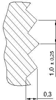
DETAIL OF KNURLS
