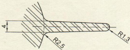
SEC. C - C SCALE 2 : 1
