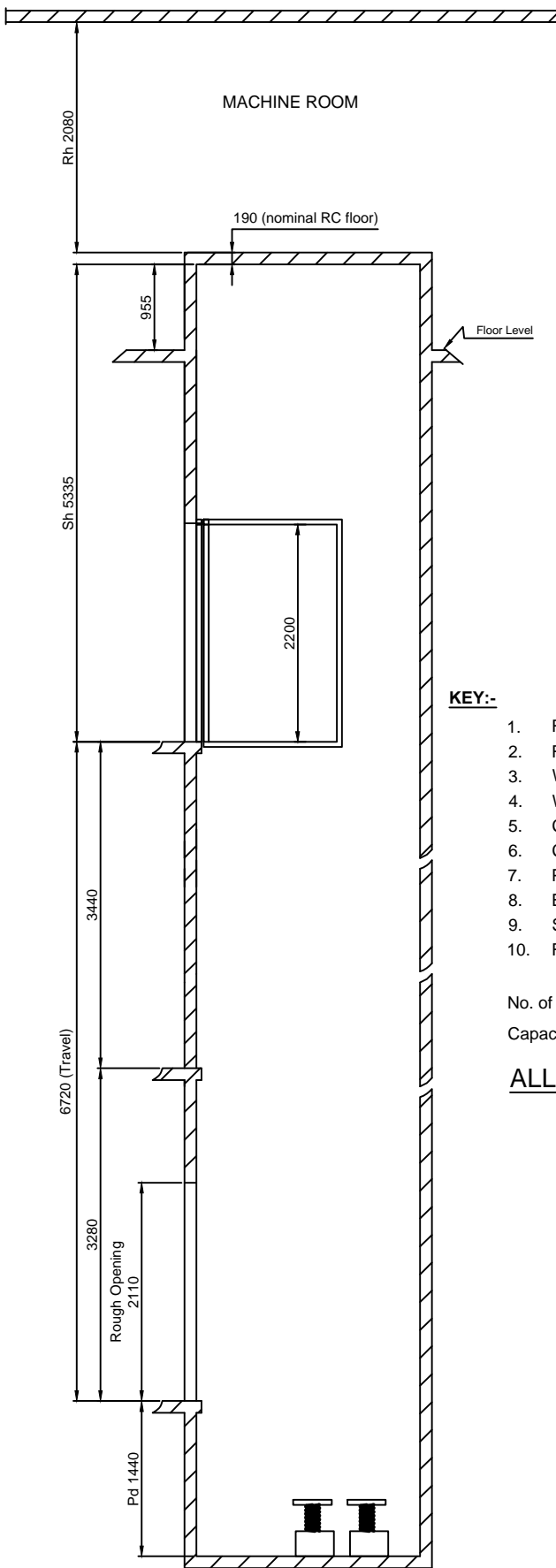
(a) Vertical section through well
