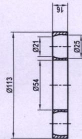
DETAIL OF SECTION A - A'
